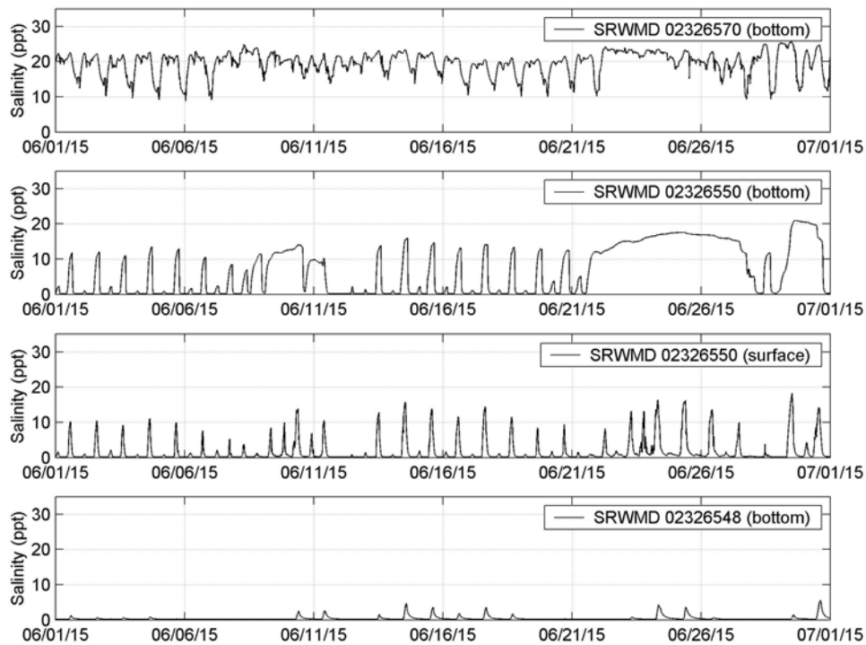
Figure 4-2e. Measured Salinity at Station SRWMD 02326570, 02326550, 02326548 (June 2015)
