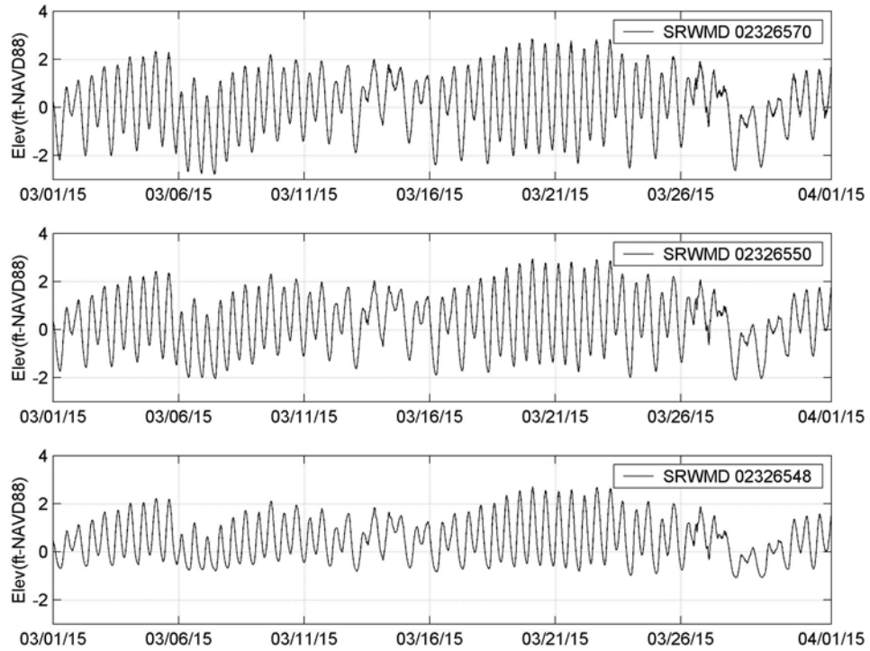
Figure 4-1b. Measured Water Level at Station SRWMD 02326570, 02326550, 02326548 (March 2015)
