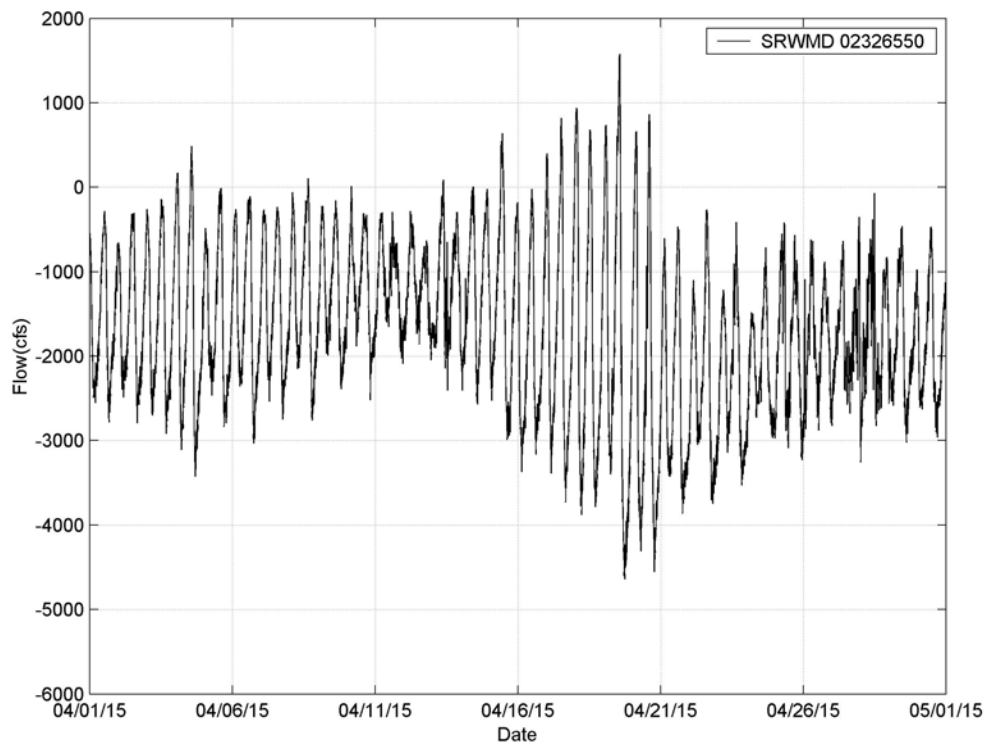
Figure 4-4c. Calculated Flow at Station SRWMD 02326550 (April 2015)
