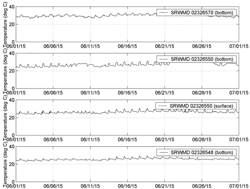
Figure 4-3e. Measured Temperature at Station SRWMD 02326570, 02326550, 02326548 (June 2015)
