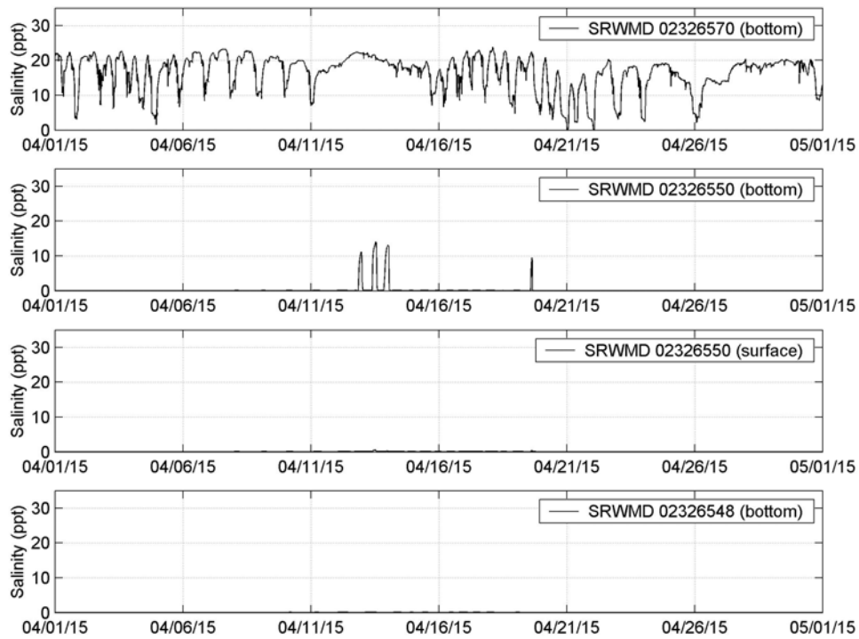
Figure 4-2c. Measured Salinity at Station SRWMD 02326570, 02326550, 02326548 (April 2015)
