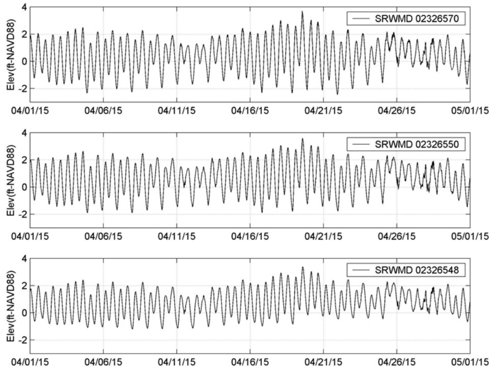
Figure 4-1c. Measured Water Level at Station SRWMD 02326570, 02326550, 02326548 (April 2015)
