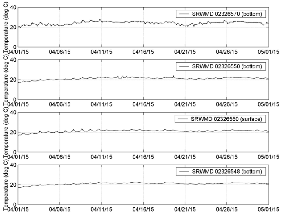
Figure 4-3c. Measured Temperature at Station SRWMD 02326570, 02326550, 02326548 (April 2015)
