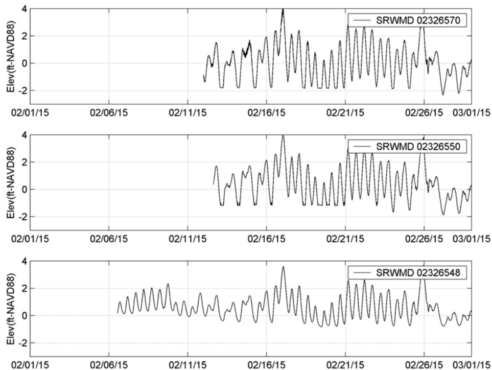
Figure 4-1a. Measured Water Level at Station SRWMD 02326570, 02326550, 02326548 (February 2015)
