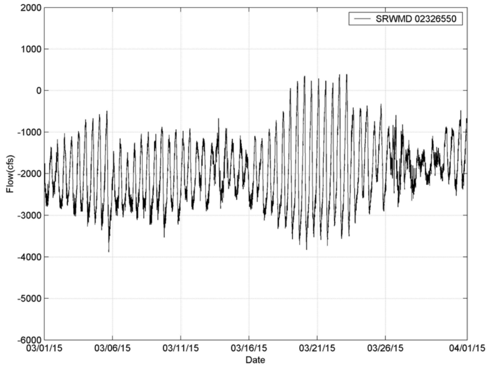
Figure 4-4b. Calculated Flow at Station SRWMD 02326550 (March 2015)
