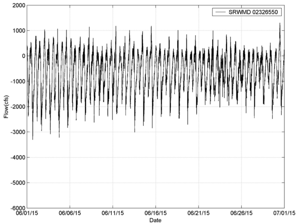
Figure 4-4e. Calculated Flow at Station SRWMD 02326550 (June 2015)
