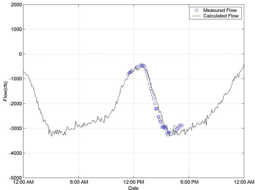
Figure 3-1. Measured and Calculated Flow on March 18, 2015
