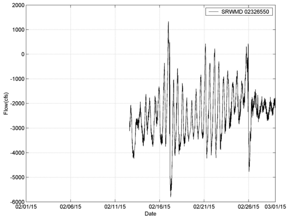
Figure 4-4a. Calculated Flow at Station SRWMD 02326550 (February 2015)
