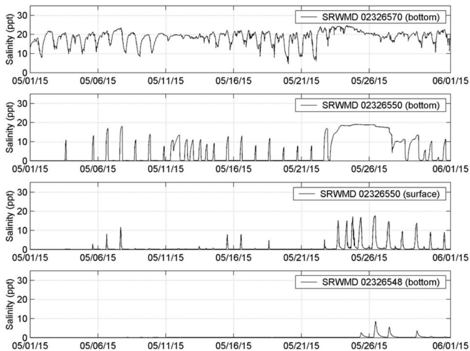
Figure 4-2d. Measured Salinity at Station SRWMD 02326570, 02326550, 02326548 (May 2015)
