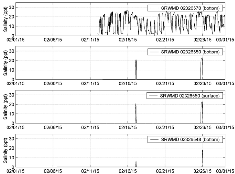
Figure 4-2a. Measured Salinity at Station SRWMD 02326570, 02326550, 02326548 (February 2015)
