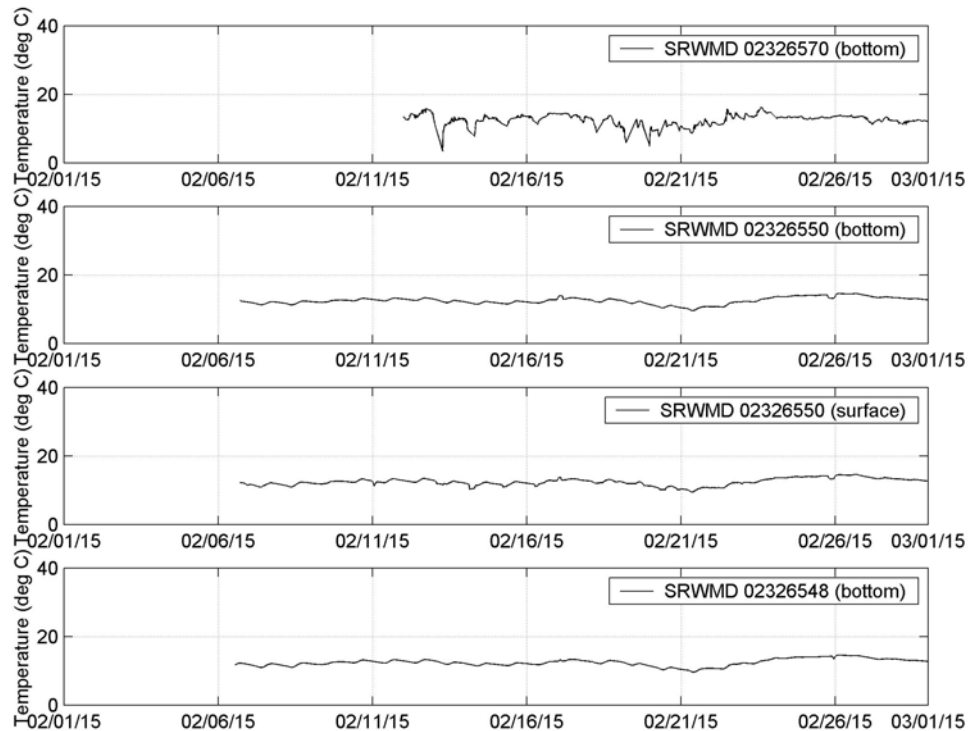
Figure 4-3a. Measured Temperature at Station SRWMD 02326570, 02326550, 02326548 (February 2015)
