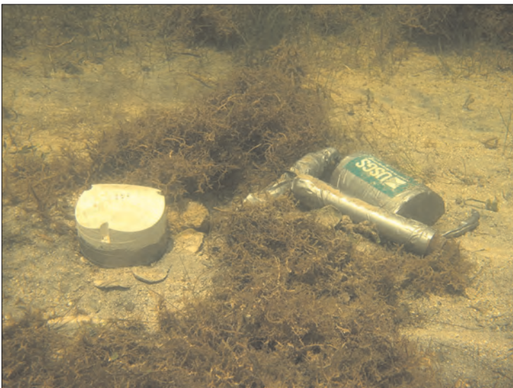
Figure 1-14. Uplooker ADVM on the streambed with biofouling paint applied. (Photograph by Victor Levesque, USGS.)
