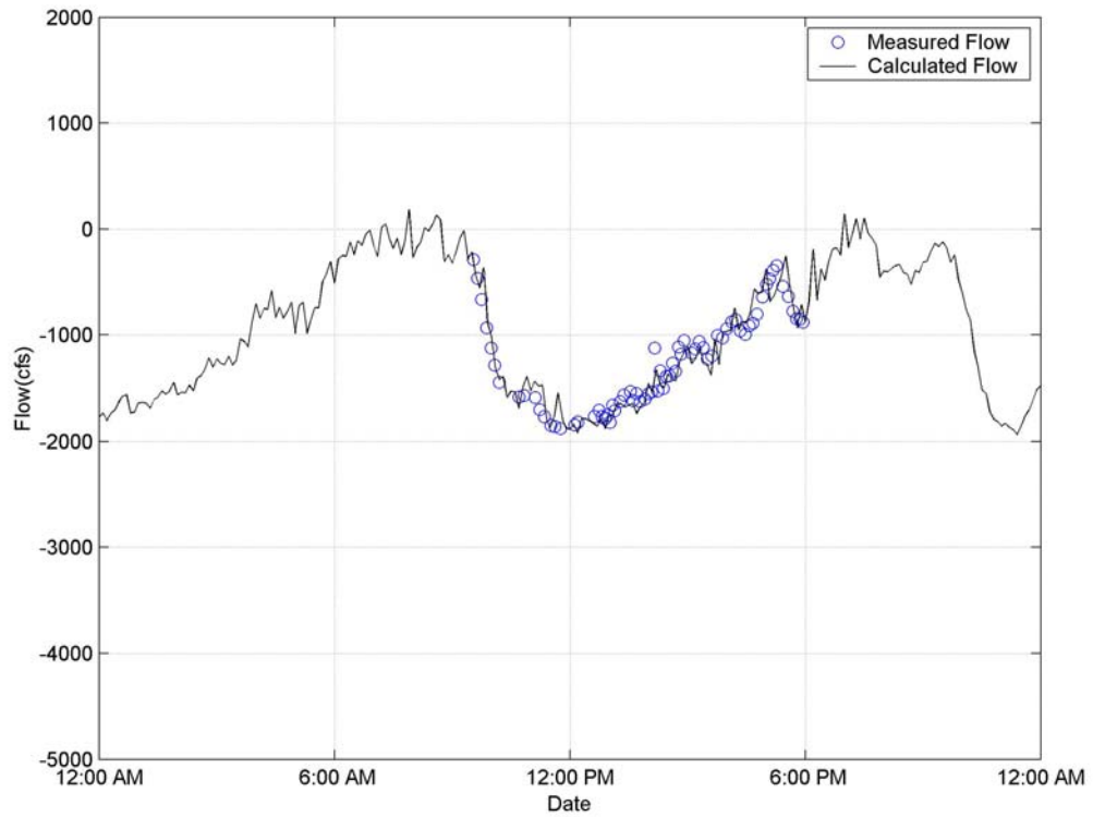
Figure 3-2. Measured and Calculated Flow on May 12, 2015
