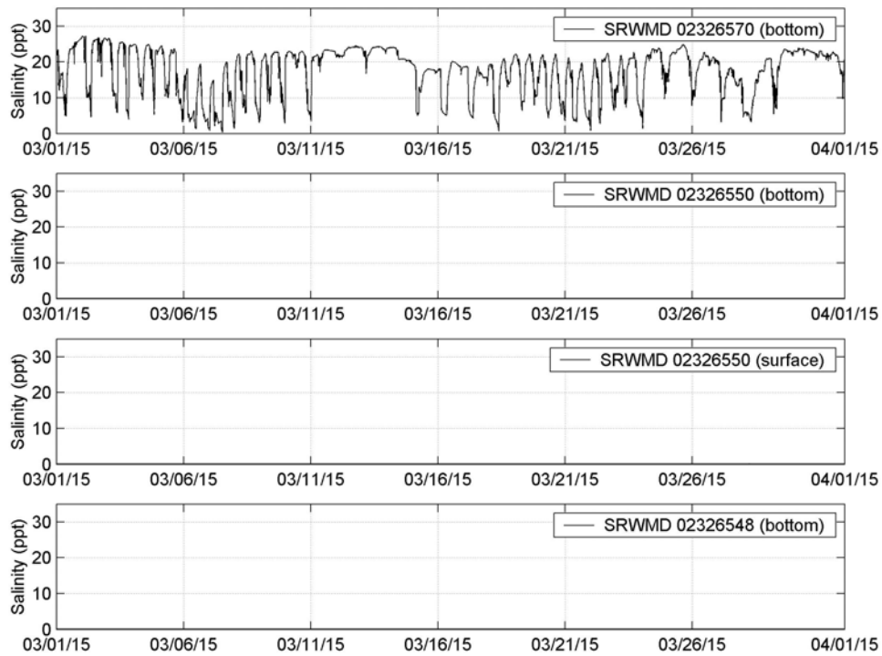
Figure 4-2b. Measured Salinity at Station SRWMD 02326570, 02326550, 02326548 (March 2015)
