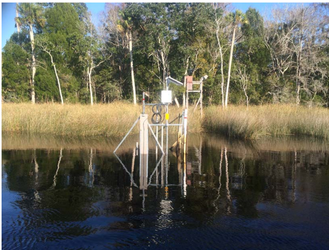
Figure 2-4. Photo of Mid Station Installation (SRWMD 02326550)
