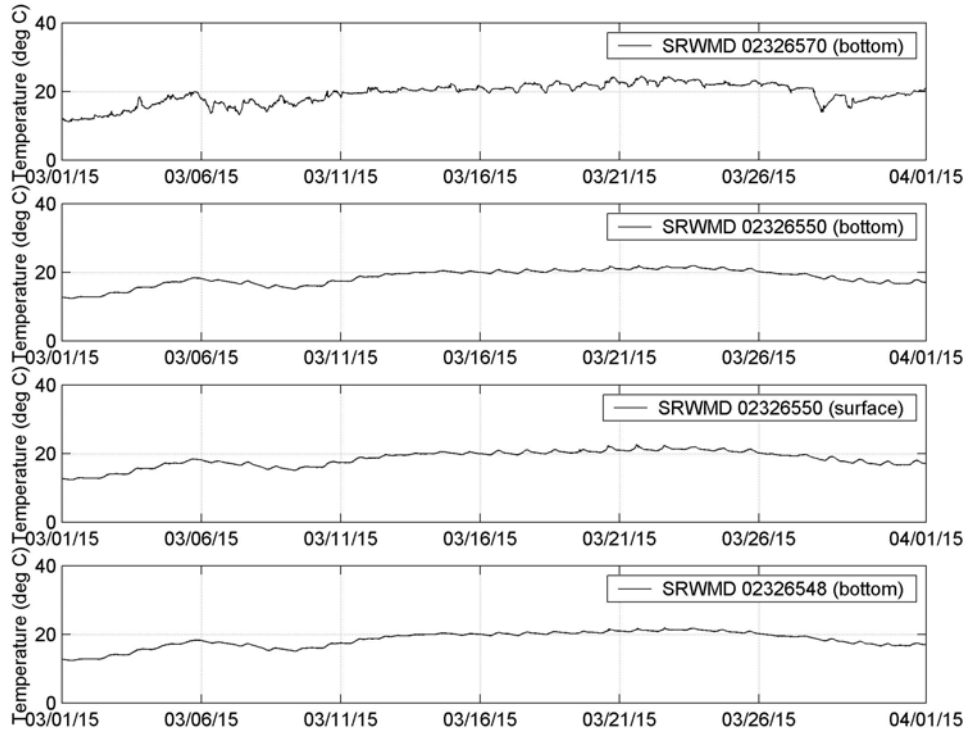
Figure 4-3b. Measured Temperature at Station SRWMD 02326570, 02326550, 02326548 (March 2015)
