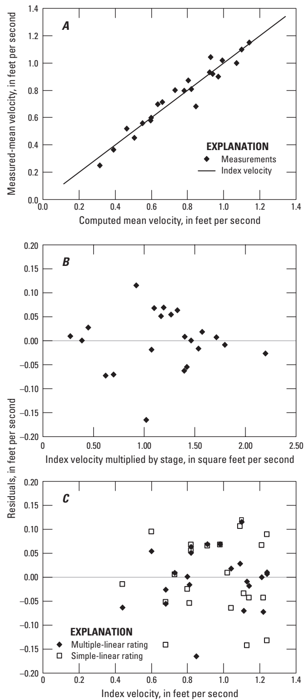
Figure 40. Plots of (A) measured-mean velocity with computed mean velocity and residuals with (B) stage multiplied by index velocity and (C) index velocity for multiple-linear regression using index velocity and stage multiplied by index velocity as independent variables.
