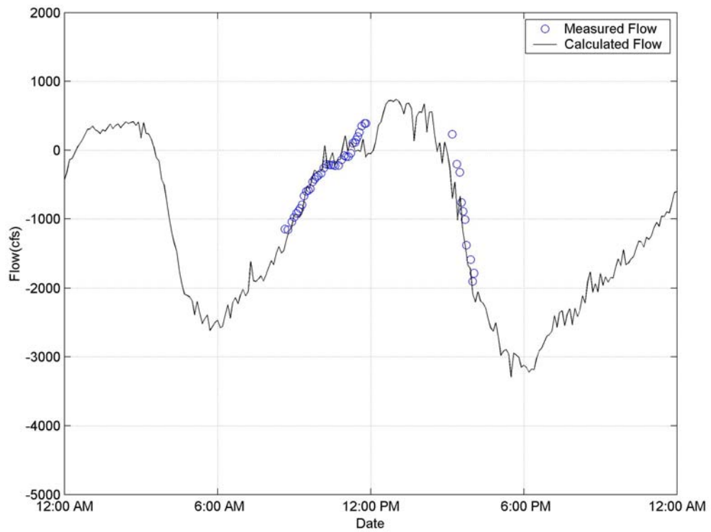
Figure 3-3. Measured and Calculated Flow on May 19, 2015
