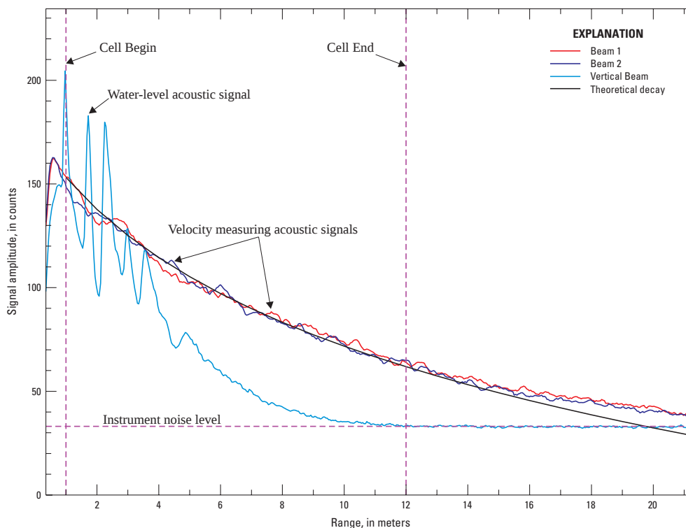
Figure 3-1. Results of a sample beam (signal amplitude) check for a sidelooker ADV with a water-level acoustic beam.
