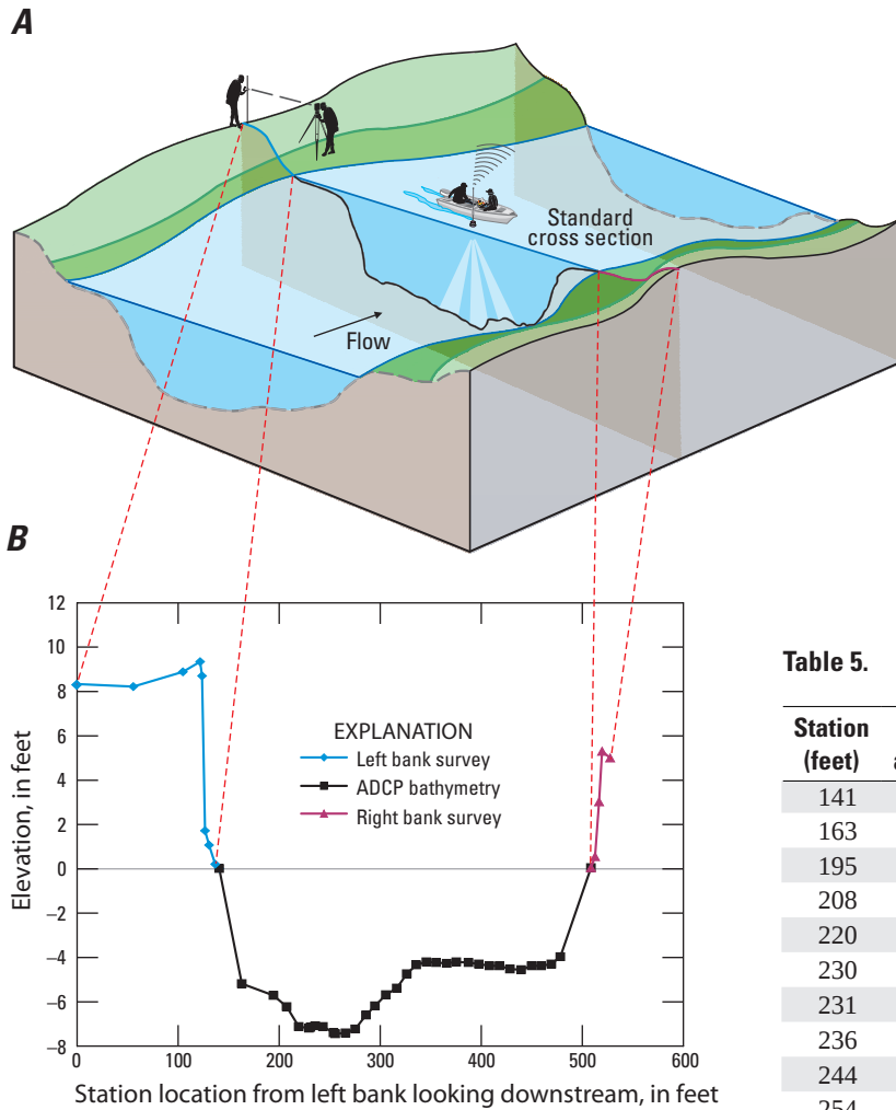
Figure 19. Combined stage-area survey created from (A) standard surveying techniques on shore (table 4) and a vessel-mounted acoustic Doppler current profiler (ADCP) used to capture channel bathymetry along measured cross sections (table 5) and (B) cross section derived from combined shore survey with ADCP channel bathymetry (diagram modified from Ruhl and Simpson, 2005).
