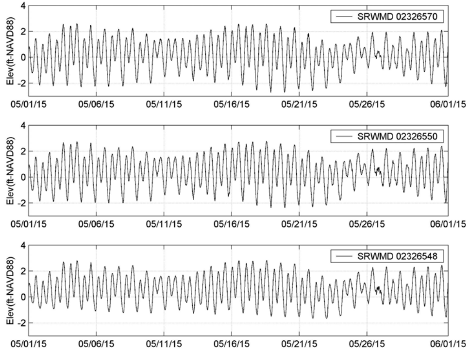
Figure 4-1d. Measured Water Level at Station SRWMD 02326570, 02326550, 02326548 (May 2015)
