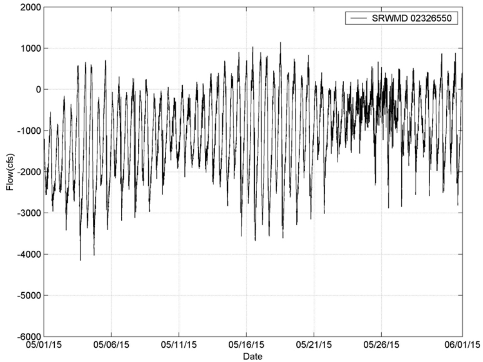
Figure 4-4d. Calculated Flow at Station SRWMD 02326550 (May 2015)
