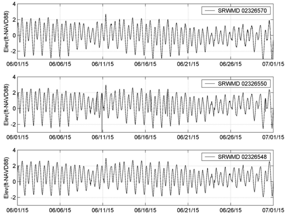
Figure 4-1e. Measured Water Level at Station SRWMD 02326570, 02326550, 02326548 (June 2015)
