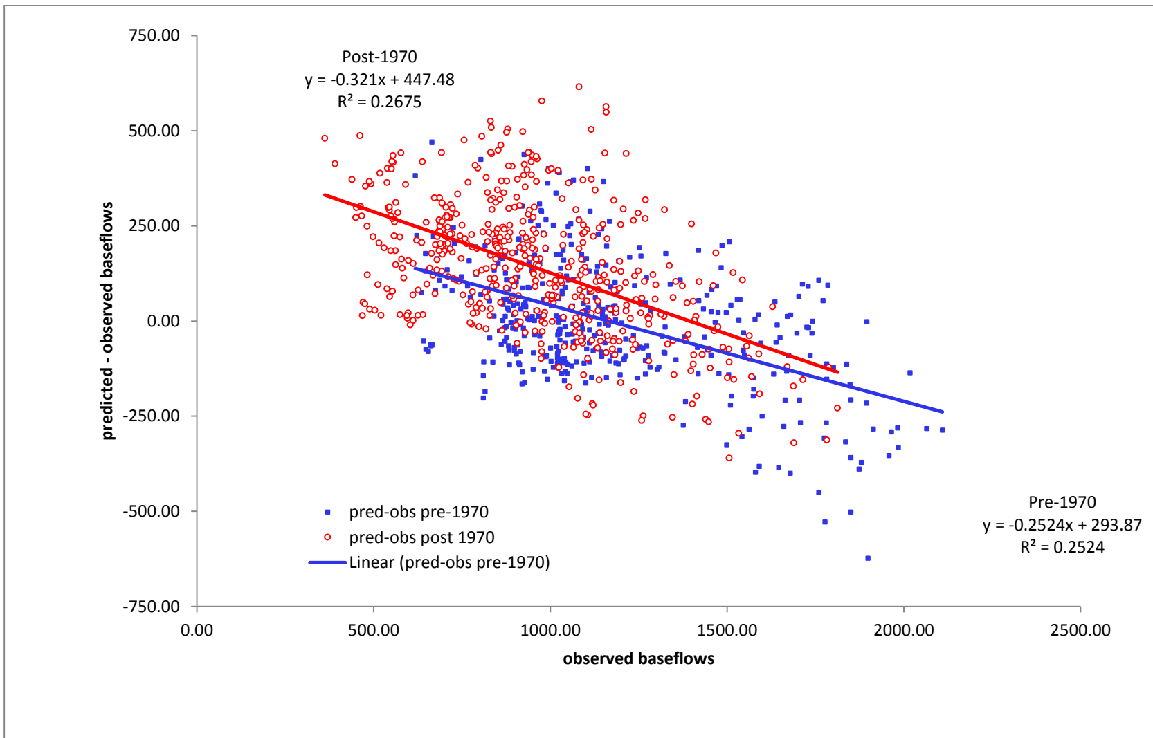
Figure 7: Magnitude of MLR residuals as a function of baseflow. Low flows are systematically over predicted and high flows are systematically under predicted for both the pre and post-1970 periods
