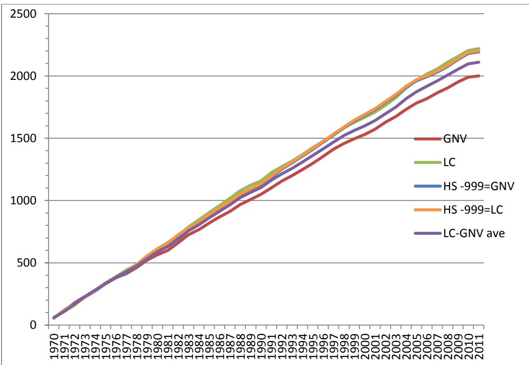
Figure 2. Cumulative rainfall from 1970 to 2011 for Lake City (LC), High Springs (HS), Gainesville (GNV) and the average of the Lake City and Gainesville (LC-GNV ave) rain gauges. The High Springs data gaps were filled with both Gainesville gage data (HS -999 = GNV) and Lake City gage data (HS -999 = LC).
